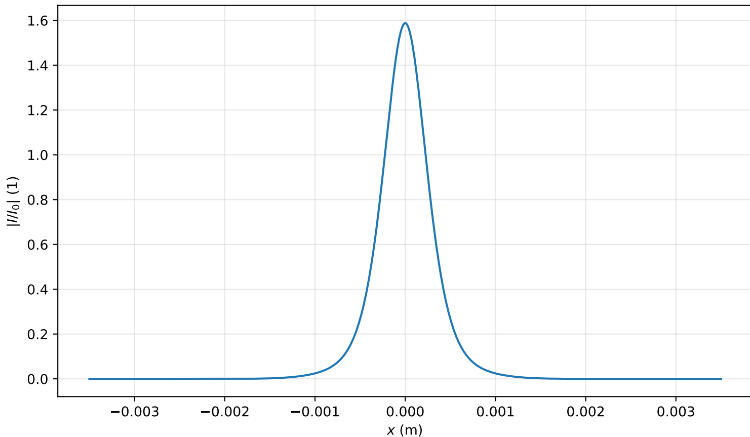
Intensity profile I(x, y = 0, z = 1.592m)/I_0 , P_{in}=0.9P_{cr} , artificial time
